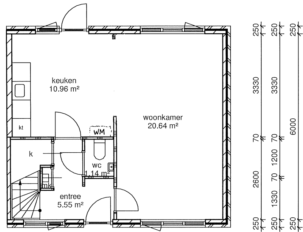
170 3290 90 3440 250 110 1340 70 920 70 950 90 3440 250 110 6880 250 begane grond
